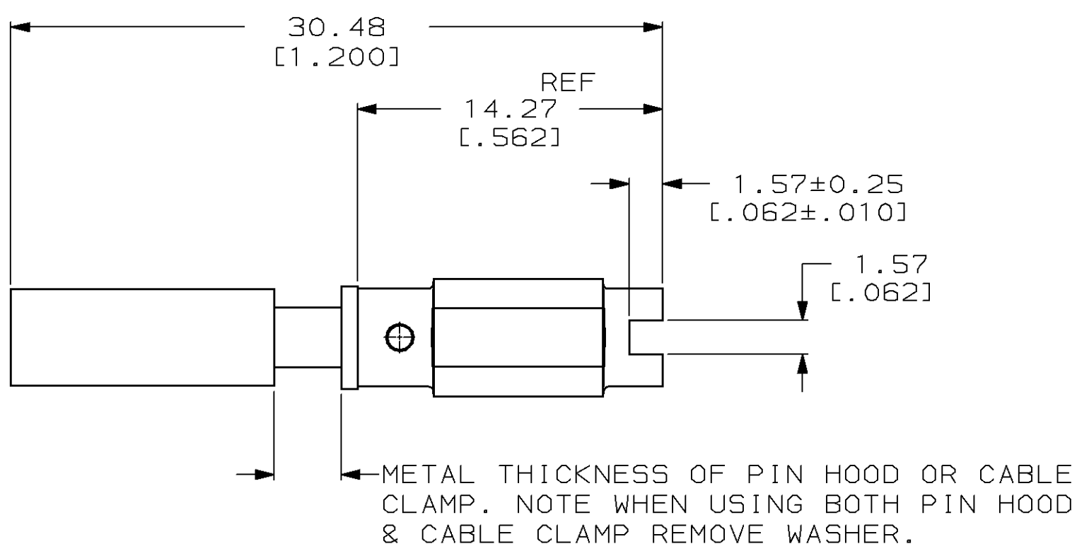
ASSEMBLED VIEW
